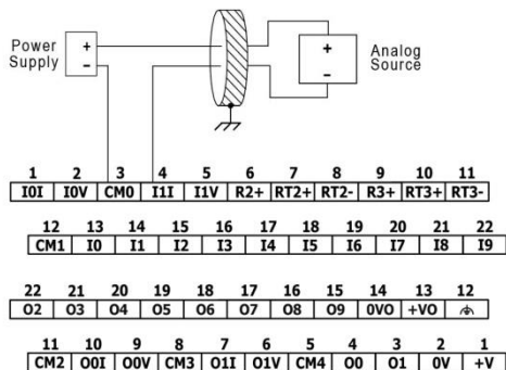
2-wire
