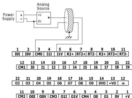
Single-ended
