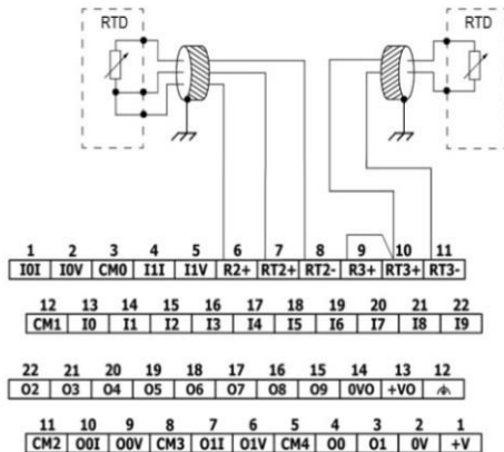
3-wire and 2-wire
