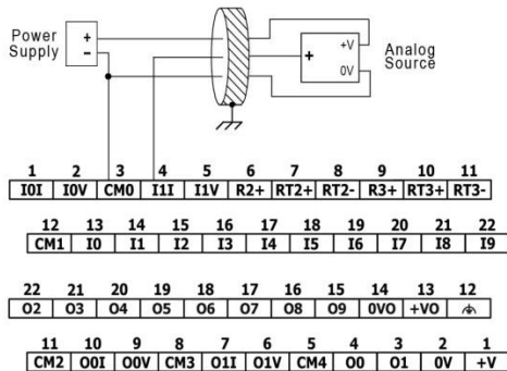
4-wire
