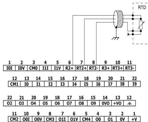
4-wire
