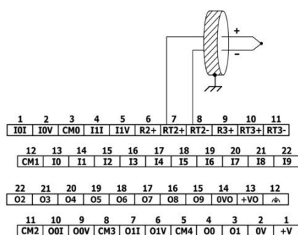
Thermocouple
