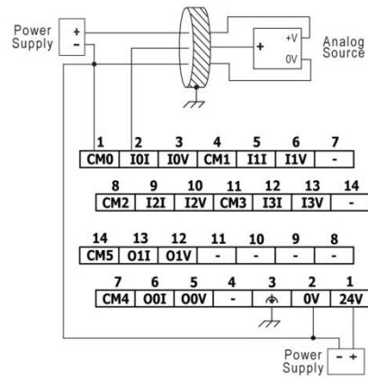
3-wire
