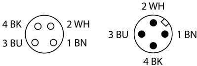
Circuit Diagram
