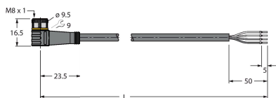
Dimension drawing Type ID no.
