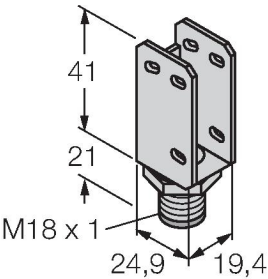
Mounting bracket, stainless steel, for 18 mm thread
