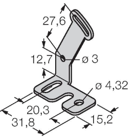
Mounting bracket, stainless steel, for 18 mm thread
