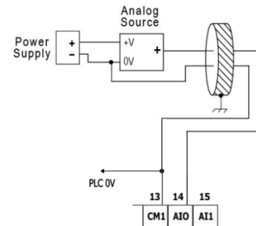
Single-ended
