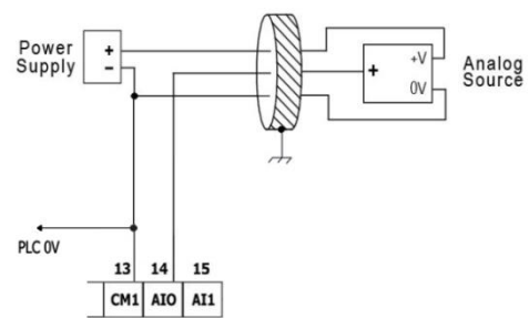
3-wire
