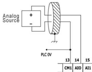
Differential
