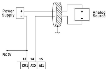
2-wire
