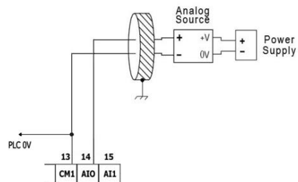
4-wire
