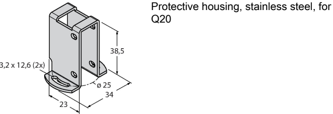
Mounting bracket, stainless steel, rectangular, for Q20
